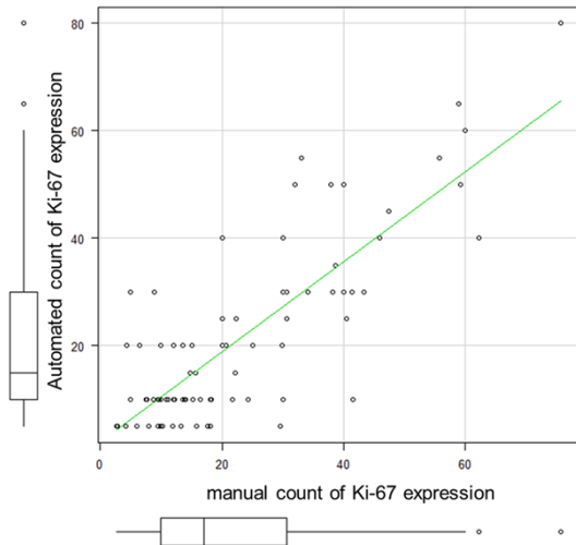
Figure 2. The automated and manual assessment of the identical fields is plotted. Solid line automated Ki-67 counts indicated a positive correlation with the manual count of Ki-67 positive cells (Pearson r = 0.816 , P < 0.001 ).
